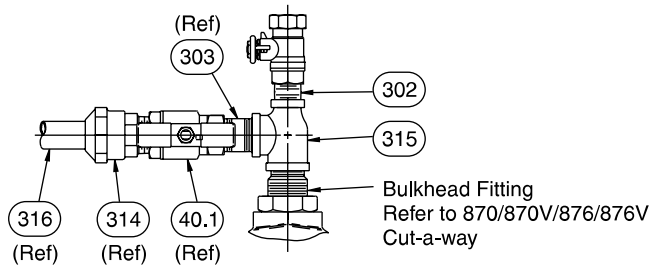
VIEW B-B (Inlet side of valve)
