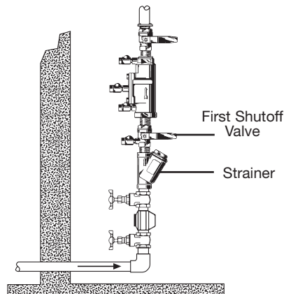
007QT-S Vertical flow-up or vertical flow-down installation (flow-up shown)
