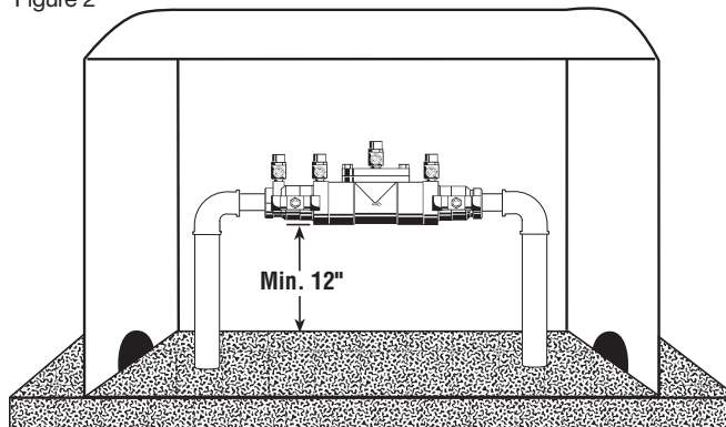
Fiberglass WattsBox
