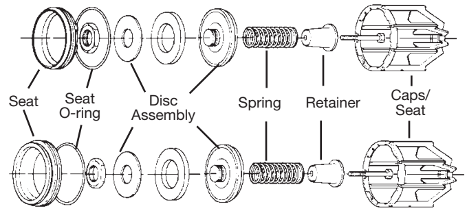
Check Assemblies
